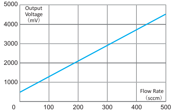
Figure 1.1: The typical analog output curve of full scale 500 sccm.
