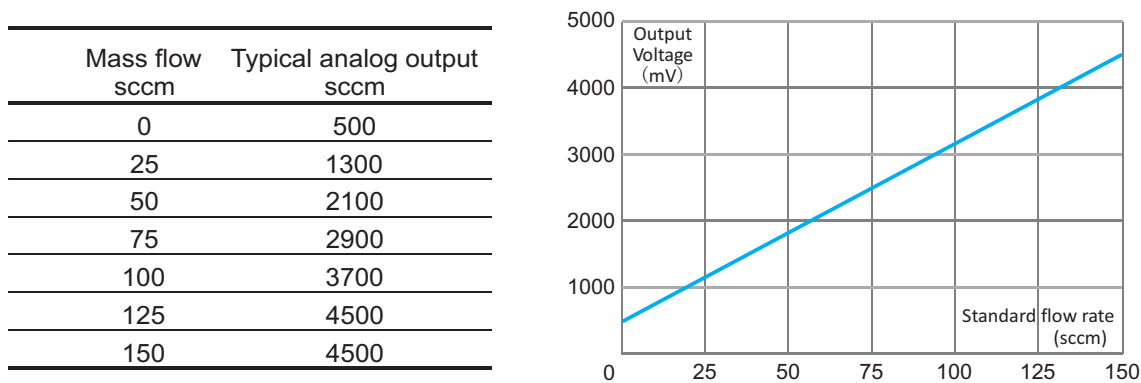
Figure 1.1: The typical analog output curve of full scale 150 sccm.
