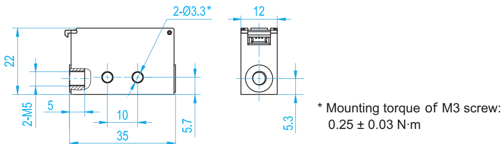
Figure 3.1: The FS8001 mechanical dimensions.
