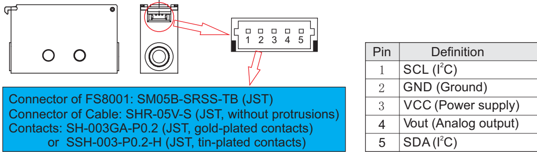
Figure 2.1: FS8001 pin configuration.
