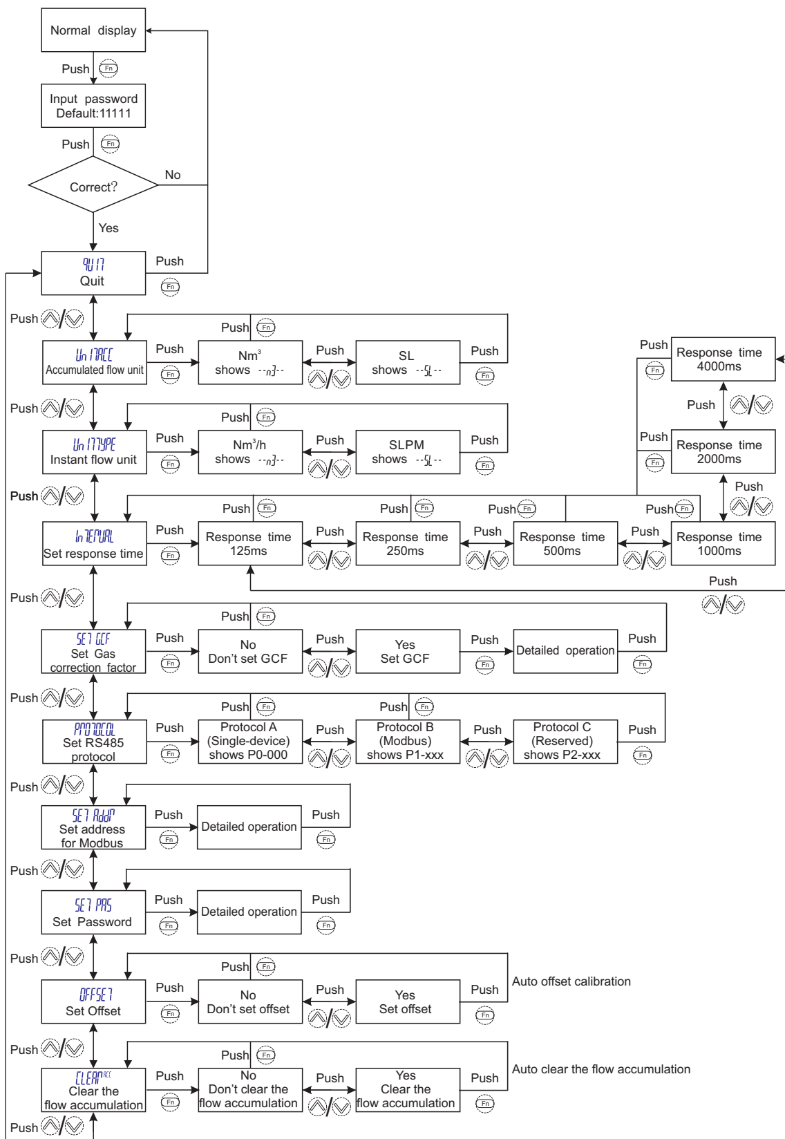
Figure 6-11 Button operation
